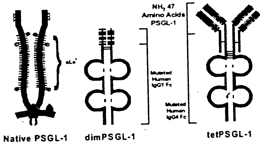
Structure of PSGL-1 Molecules
